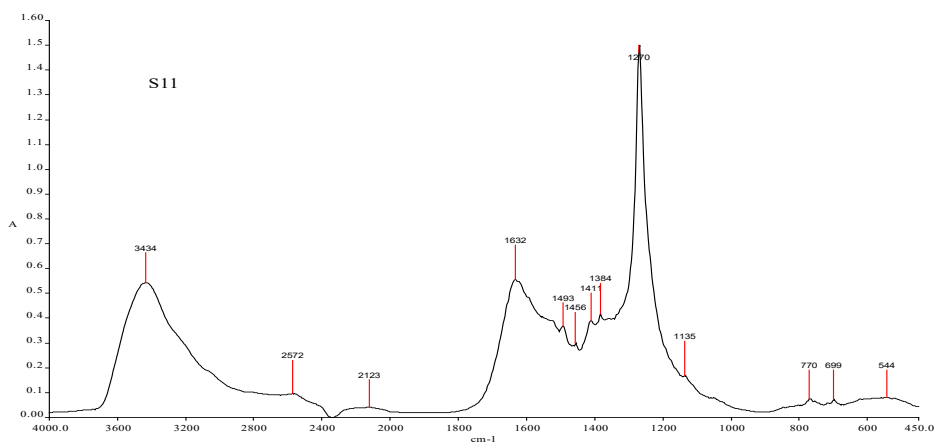
Figure 4. IR spectrum of the ligand
