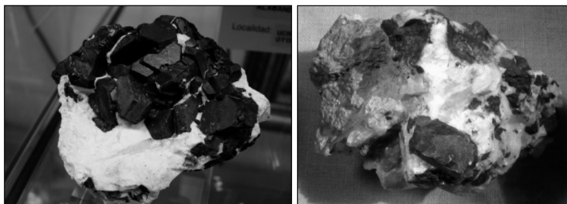
Figure 4. Alabandite or alabandine, (\text{dMnS})
