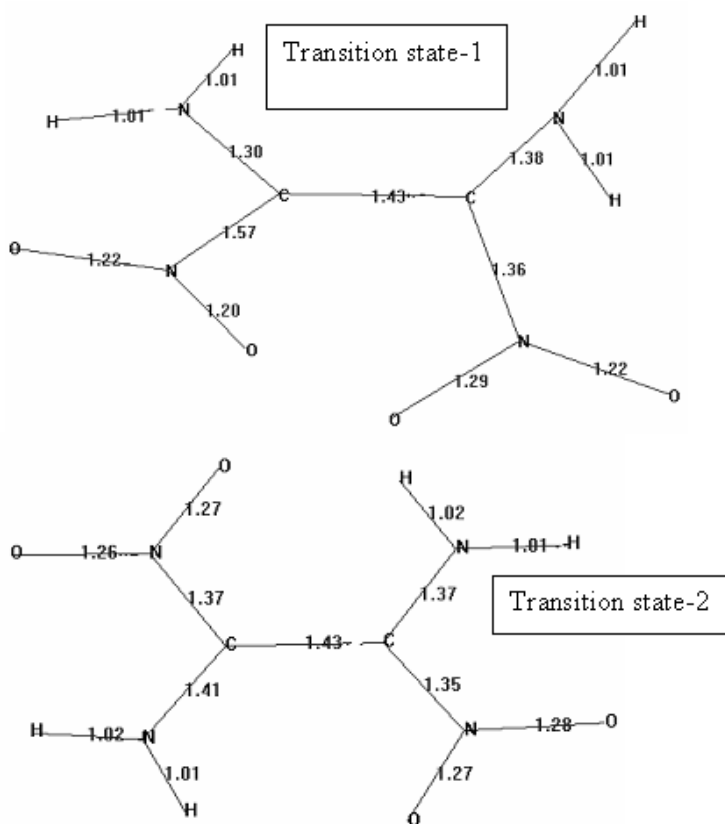
Figure 13. Bond lengths (Å) in transition states-1 and 2 (B3LYP/6-311++G(d,p))
