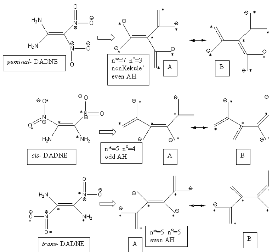
Figure 9. The isoconjugate systems of DADNE isomers
