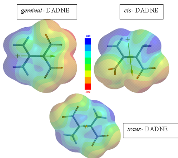
Figure 7. Electrostatic potential maps of the isomers considered (B3LYP/6-311++G(d,p))
