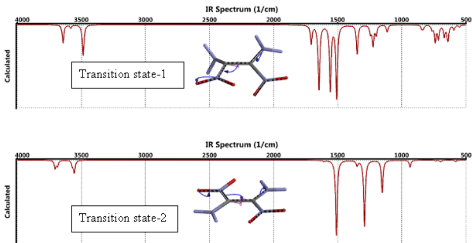
Figure 15. IR spectra of transition states 1 and 2 (B3LYP/6-311++G(d,p))
