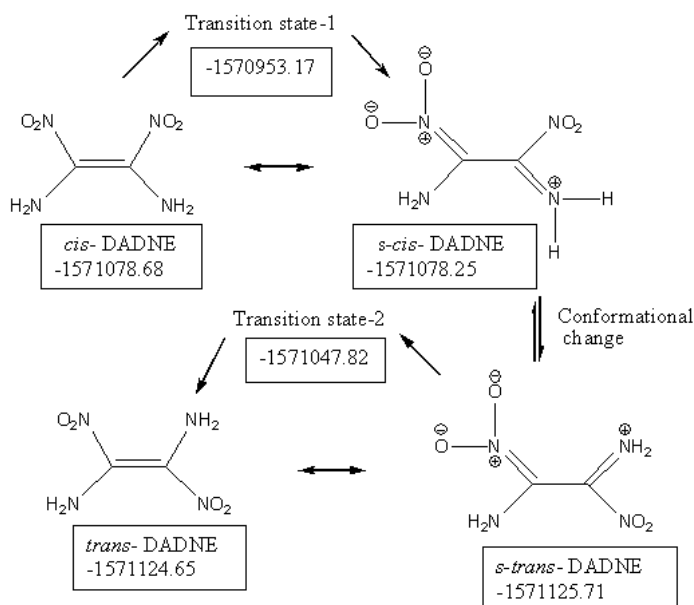
Figure 10. A possible route to the cis/trans isomerization considered (Energies in kJ/mol. B3LYP/6-311++G(d,p))
