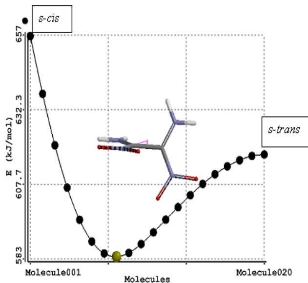
Figure 11. Conformational energy variation for s-cis - DADNE to s-trans - DADNE conversion
