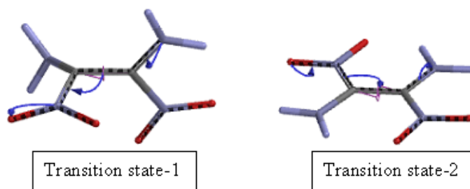
Figure 12. The shift of electrons leading to the transition state geometries (B3LYP/6-311++G(d,p))
