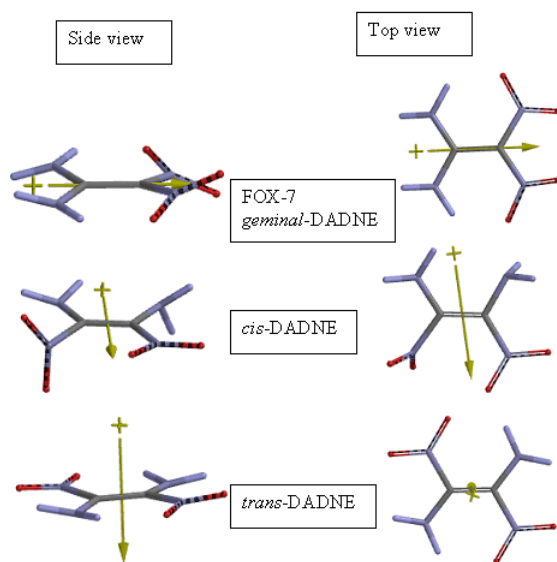
Figure 1. Optimized structures of the present concern B3LYP/6-311++G(d,p)
