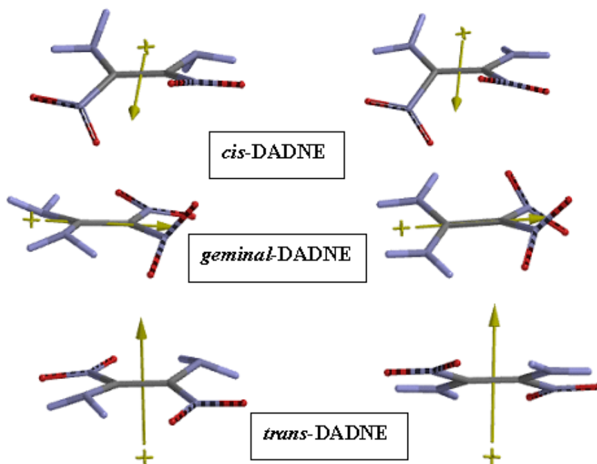
Figure 16. Optimized structures of DADNE ions (UB3LYP/6-311++G(d,p))
