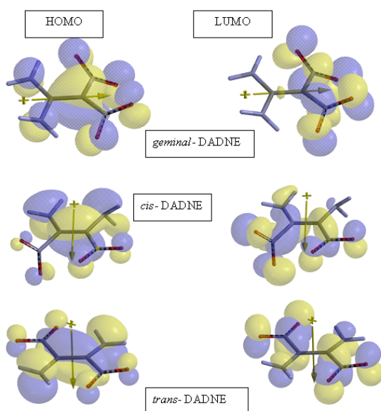
Figure 6. The HOMO and LUMO patterns of the isomers considered (B3LYP/6-311++G(d,p))
