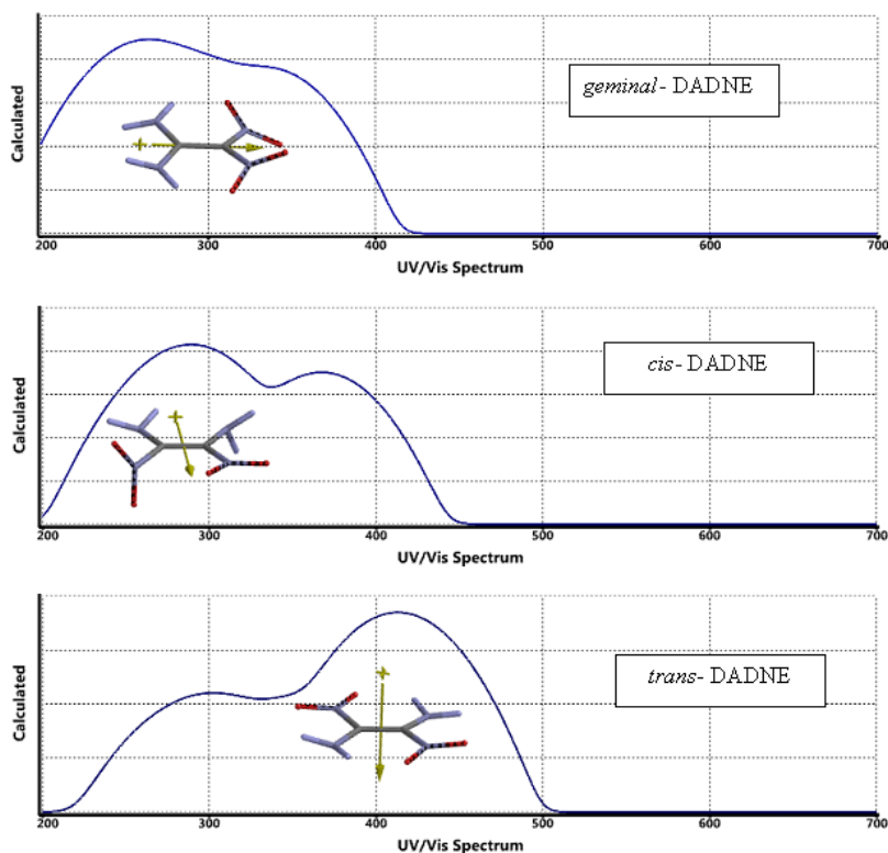
Figure 8. UV-VIS spectra of the isomers (B3LYP/6-311++G(d,p))
