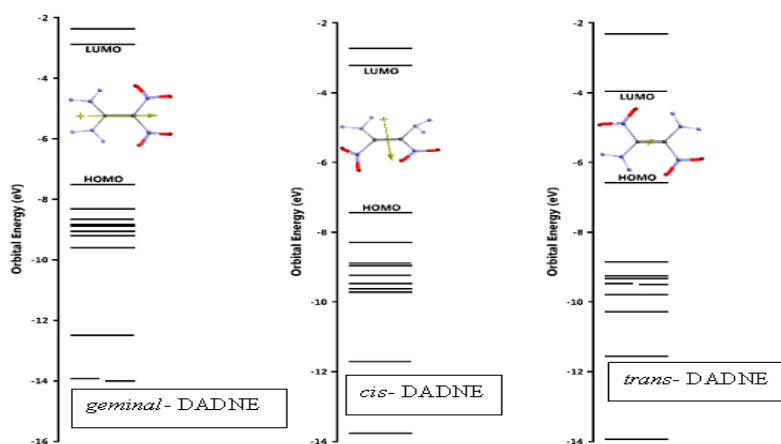
Figure 5. Some of the molecular orbital energy levels of the isomers considered (B3LYP/6-311++G(d,p))
