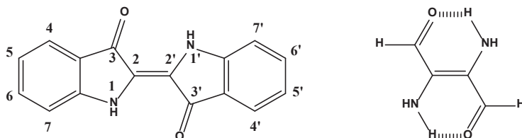
Fig. 1. Sketch of indigo (left) with the numbering position and its H-like chromophore (right) (Jacquemin et al., 2006)
