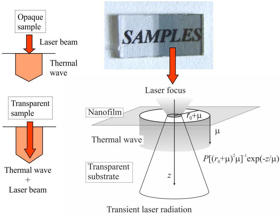
Figure 2. Sample nanofilm with PTD volume extended in the substrate confined by the superposition of thermal diffusion length and penetration depth of the laser radiation
