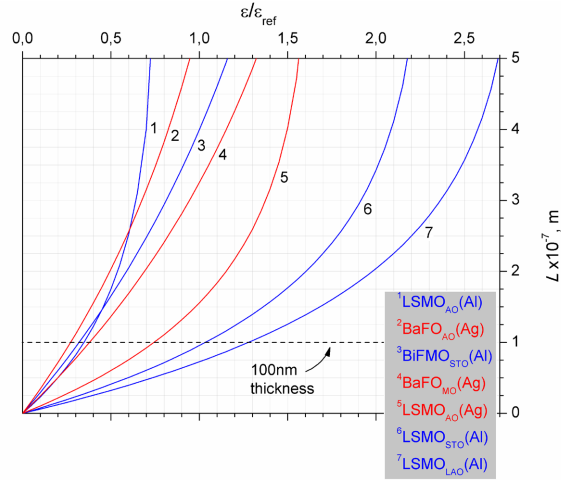
Figure 3. Evaluation of ferromagnetic and multiferroic samples on standard monocrystalline substrates numbered by lines (1 – 7) with film thickness calibrated by reference
